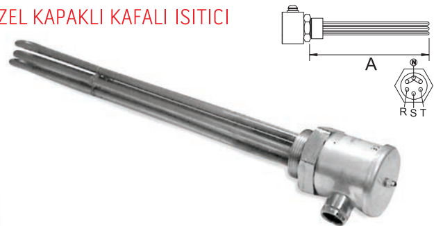
6 KW - 7.5 KW - 10 KW 1 1/2" 2" KAFALI 230-400 V
