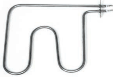
FB 11 Ø 6.5-8.5 mm Cr-Ni 230 V 800W
