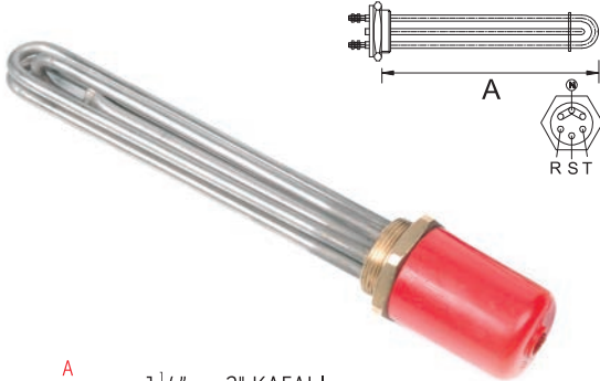
4.5 - 6 KW 350 MM 7.5 - 10 KW 435 MM 1 1/2" - 2" KAFALI 8.5 mm Cr-Ni 230-380 V
