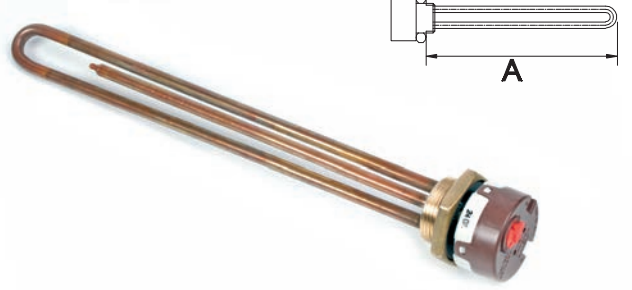
1 1/4" TERMOSTADLI ISITICI 2000 W - 2500 W 8.5 mm Cr-Ni 300 mm
