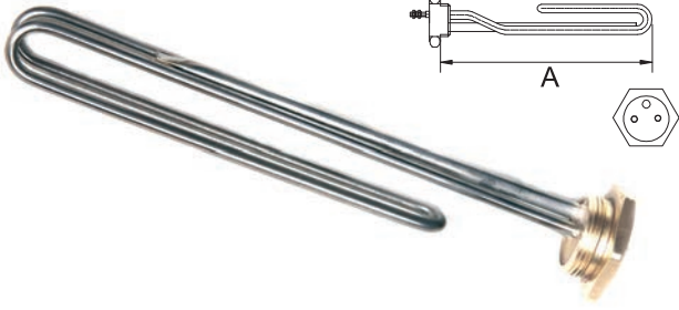
1 1/4" Ø REKORLU 2000 W - 2500 W 8.5 mm Cr-Ni 300 mm
